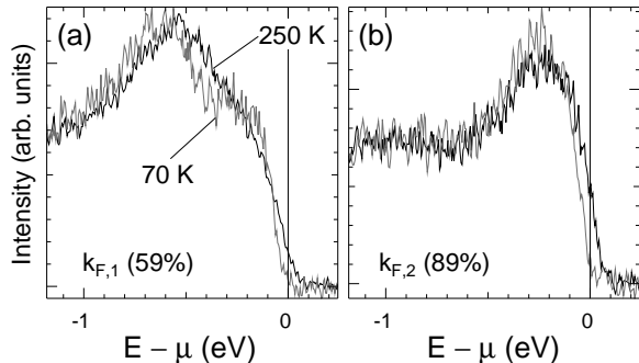
Figure 17: T dependence of spectra at FS crossings for the K_{0.3}\text{MoO}_3 data of Fig. 16.
